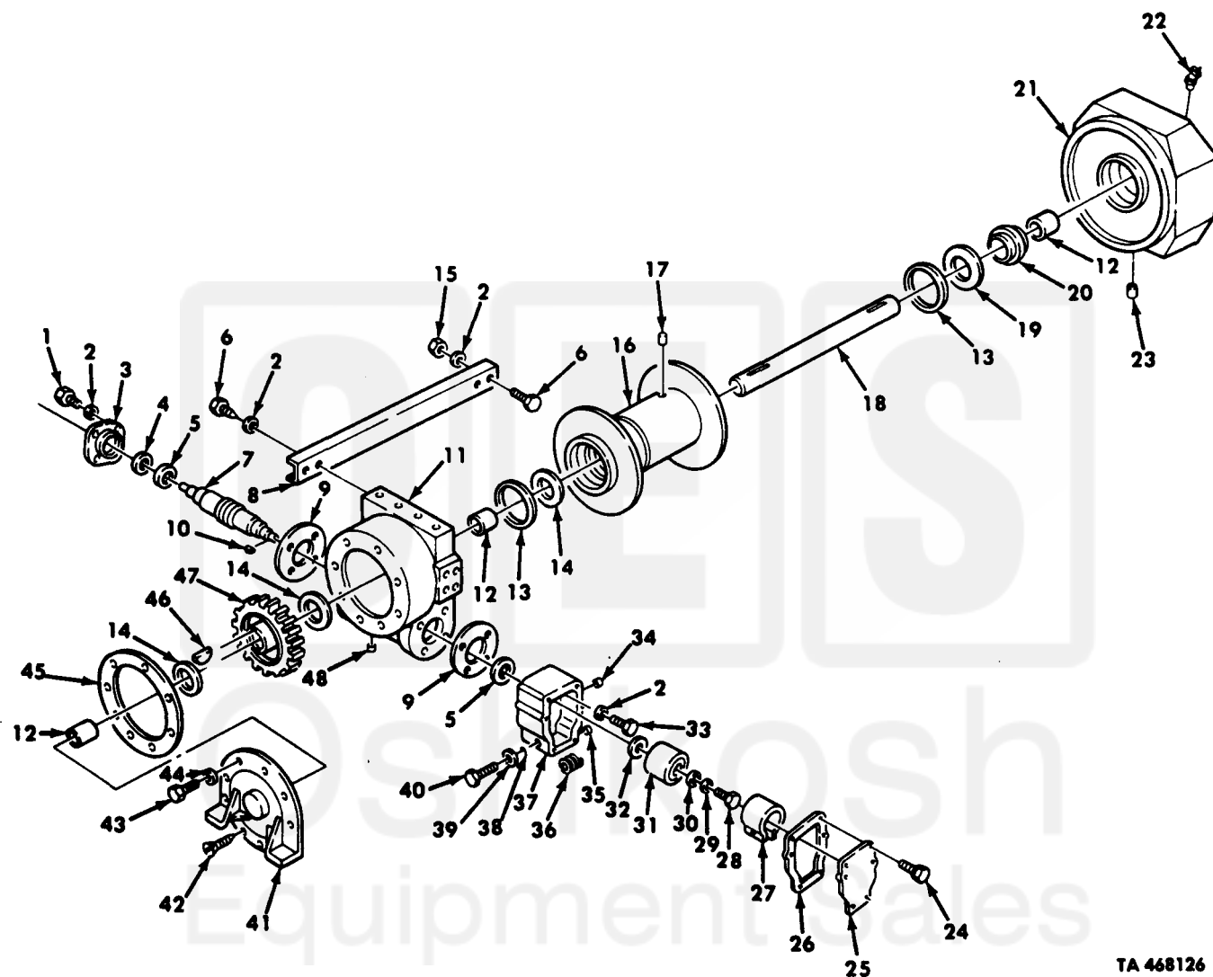
Figure 416. Wrecker Rear Winch Assembly, Basic.
